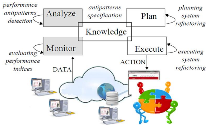
Figure 1: Antipattern-based MAPE process.
