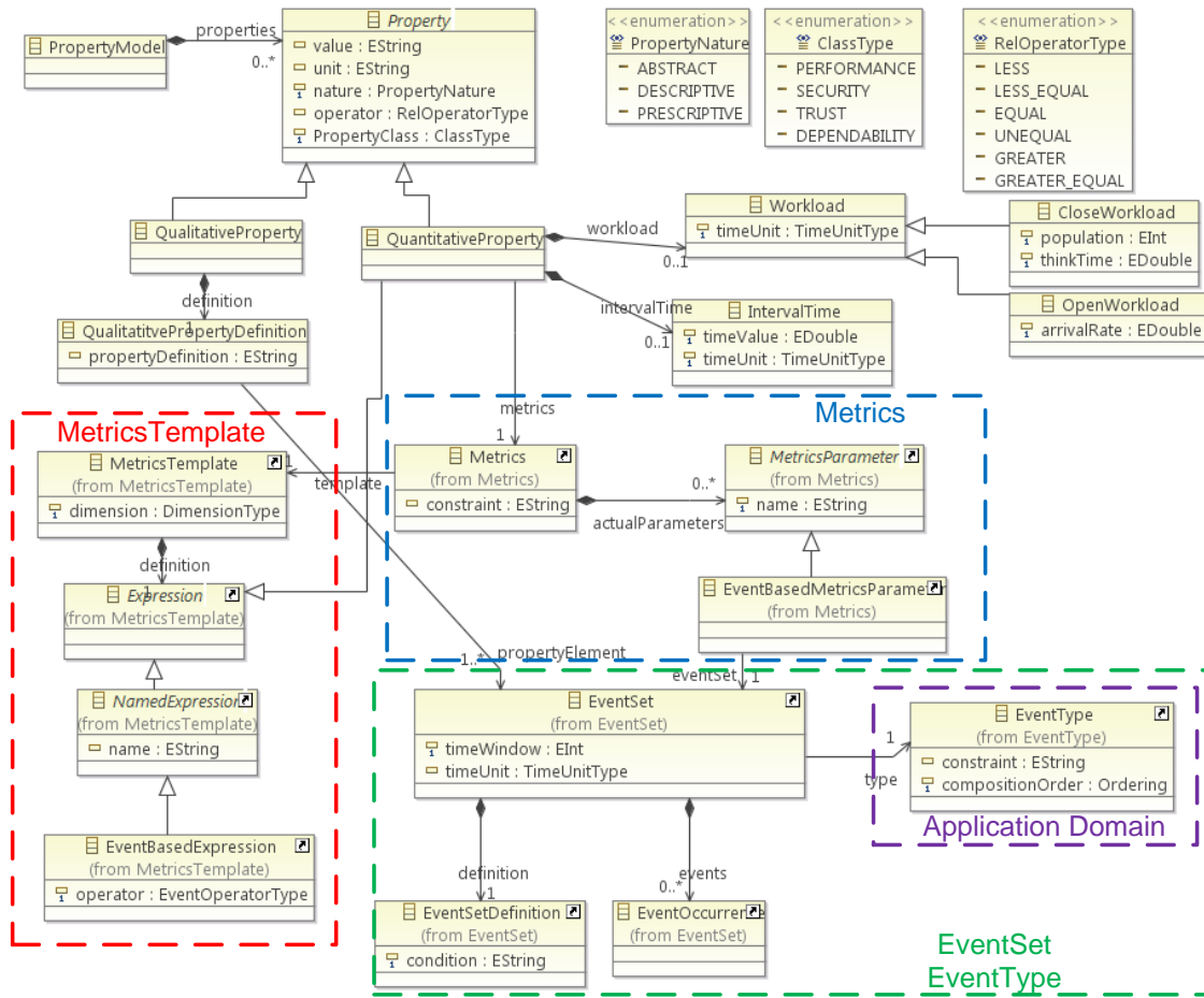
Figure 5: PMM structure.
