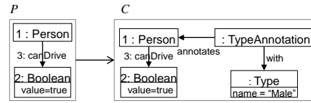
Figure 12: Constraint DriverIsMale
