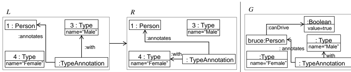
Figure 13: Left: rule FromMaleToFemale changing one's gender. Right: a situation where gender change would lead to violate constraint DriverIsMale .
