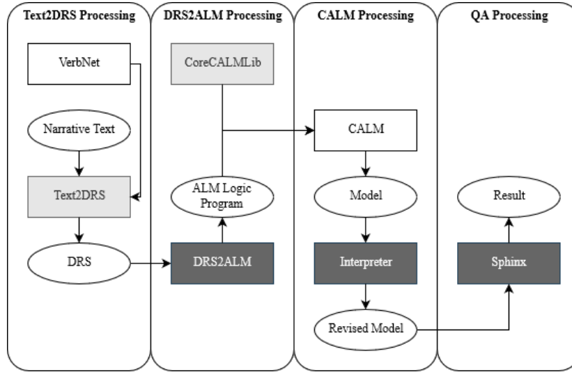
Figure 3: System TEXT2ALM Architecture
