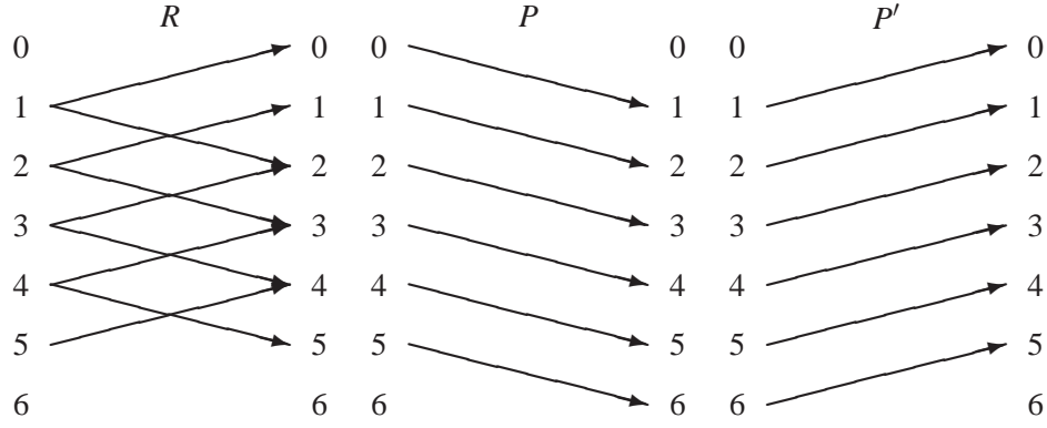
Figure 1: Enhancing Correctness Without Duplicating Behavior: P' \equiv_R P
