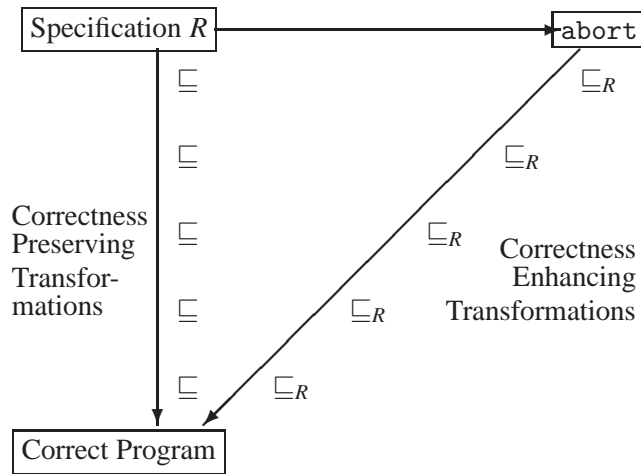
Figure 3: Alternative Program Derivation Paradigms
