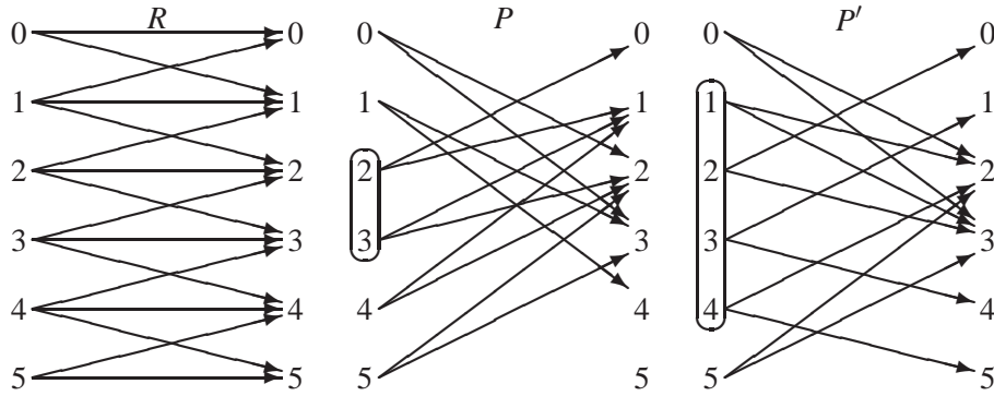
Figure 2: Relative Correctness for Non-Deterministic Programs: P' \sqsupseteq_R P .
