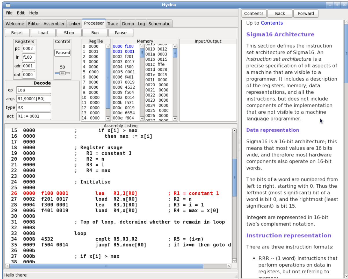
Figure 1: Hydra GUI. The Processor tab is selected, and the machine is running the ArrayMax program.
