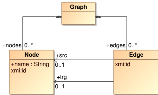
Figure 6: SimpleGraph
