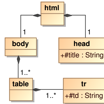
Figure 5: HtmlMetaModel
