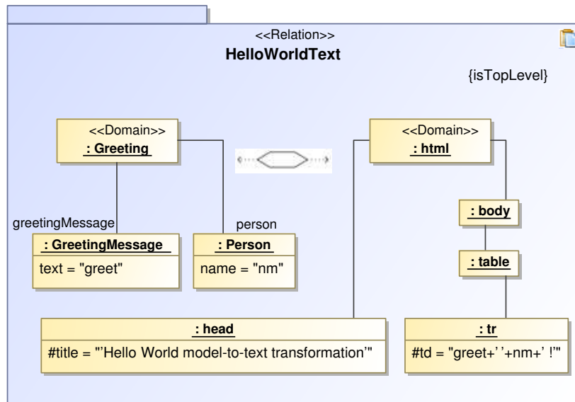
Figure 12: Model-to-text transformation
