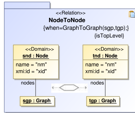
Figure 22: Starting relation—copy a graph
