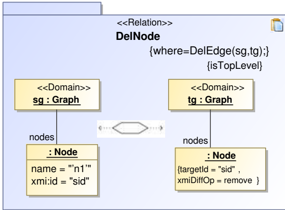
Figure 31: Delete a node with name "n1"
