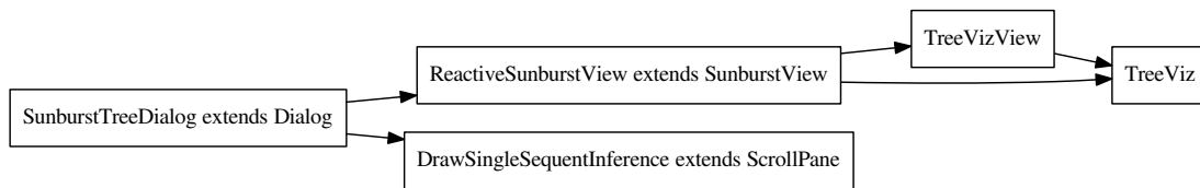
Figure 7: Architecture of SUNBURSTTREEDIALOG
