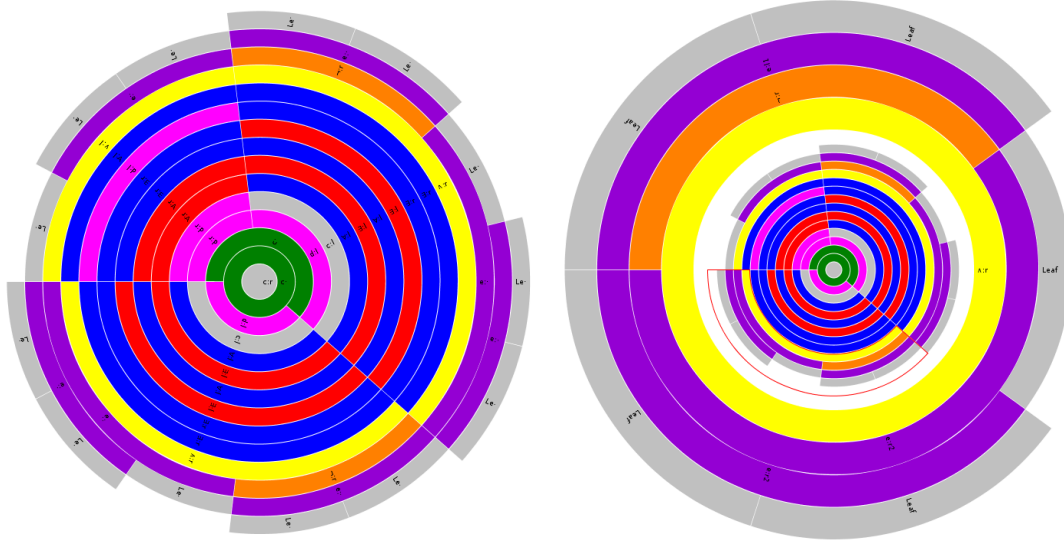
Figure 3: A combinatory proof (left) with a zoom into one of its subproofs (right).
