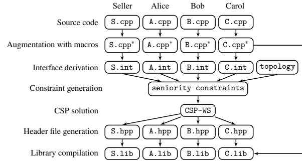
Figure 4: An interface reconciliation workflow performed by the toolchain
