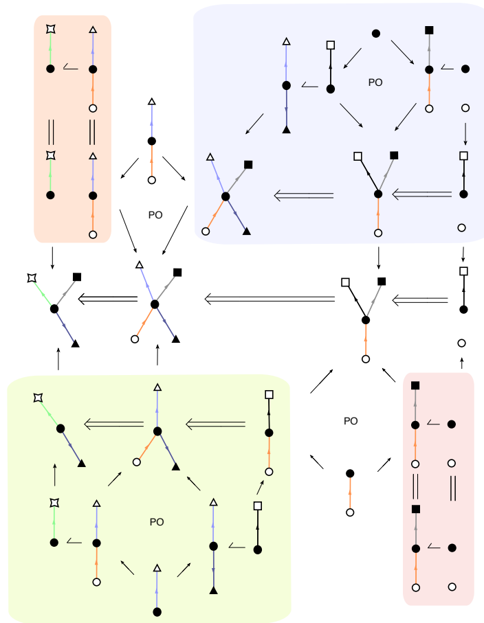
(b) Explicit demonstration of the associativity property of the rule composition operation: the top half of the diagram encodes a composition of the shape r_3 \triangleleft (r_2 \triangleleft r_3) , while the bottom half encodes (r_3 \triangleleft r_2) \triangleleft r_1 , with both operations for the overlaps depicted leading to the same minimal trace (up to isomorphisms). The tracelet of length 3 equivalently encoded by both halves of the diagram is obtained by composition of squares.
