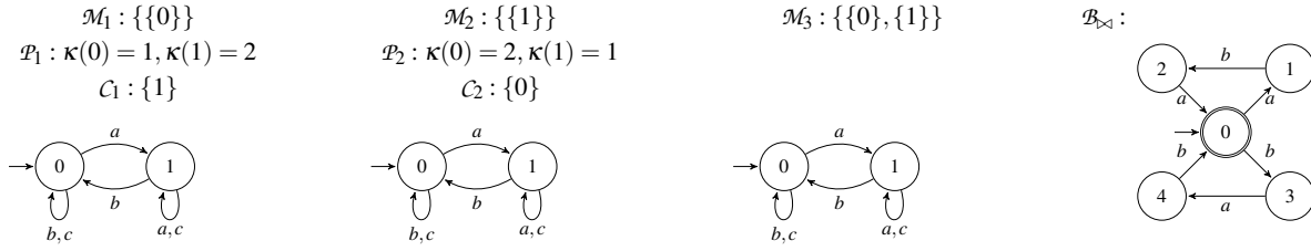
Figure 6: On the left, examples for non closure of union for \mathbb{IM} , \mathbb{IP} , and \mathbb{IC} . On the right \mathcal{B}_{\times} .
