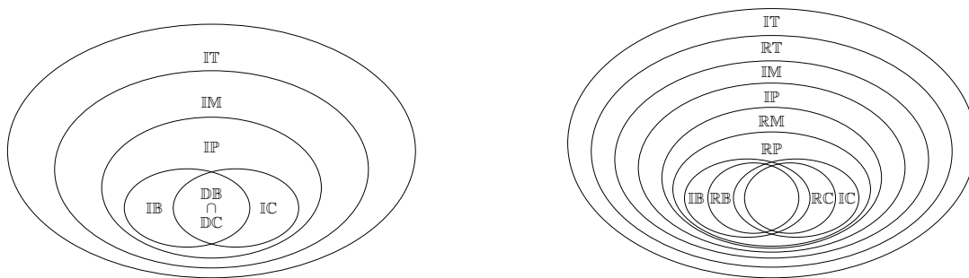
Figure 1: On the left, a summary of inclusion of the classes of \omega -automata that are isomorphic to their rightcon automaton. On the right a summary of inclusion of the classes of \omega -automata that are isomorphic to their rightcon automaton, as well as those that are in addition respective of their right congruence.
