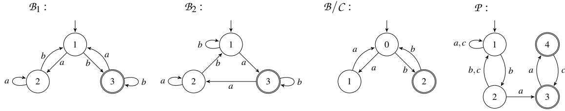
Figure 5: On the left examples for non-closure of union for \mathbb{IB} . On the right a DBA \mathcal{B} and a DCA \mathcal{C} showing \mathbb{IB} and \mathbb{IC} are not closed under complementation (the sink state is not shown).
