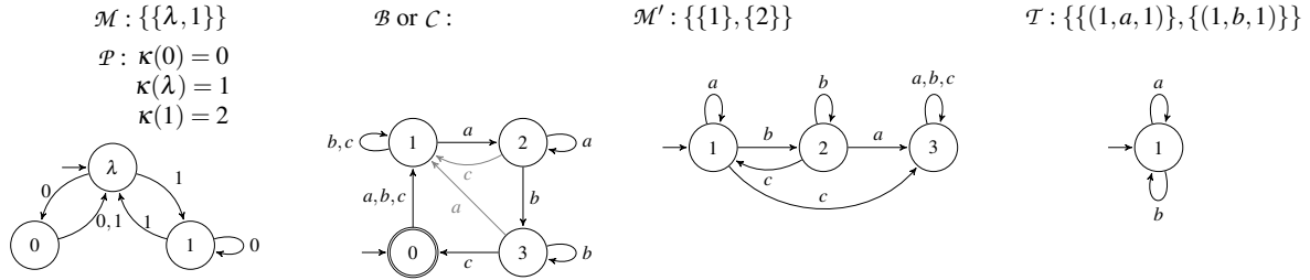
Figure 3: A DMA \mathcal{M} and an equivalent DPA \mathcal{P} for a language L_{PM} such that L_{PM} \in \mathbb{IM} \setminus \mathbb{DB} \cap \mathbb{DC} and L_{PM} \in \mathbb{IP} \setminus \mathbb{DB} \cap \mathbb{DC} . Second from the left, when regarded as a DBA \mathcal{B} we have \llbracket \mathcal{B} \rrbracket \in \mathbb{IB} \setminus \mathbb{DC} . When regarded as a DCA \mathcal{C} we have \llbracket \mathcal{C} \rrbracket \in \mathbb{IC} \setminus \mathbb{DB} . A DMA \mathcal{M}' such that \llbracket \mathcal{M}' \rrbracket \in \mathbb{IM} \setminus \mathbb{IP} , and a DTA \mathcal{T} such that \llbracket \mathcal{T} \rrbracket \in \mathbb{RT} \setminus \mathbb{RM} .
