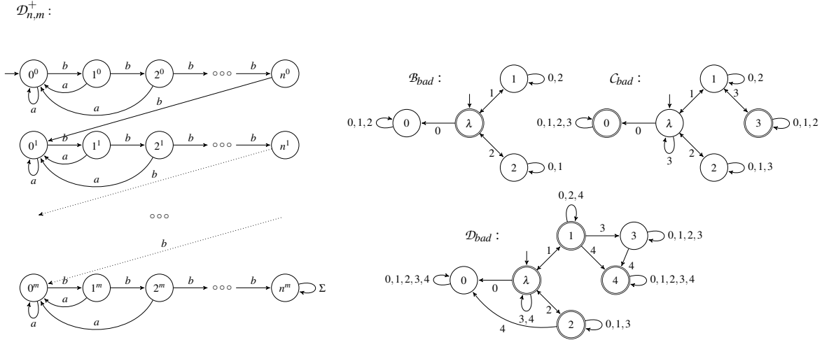
Figure 4: On the left, a representative example for the Wagner class \mathbb{DM}_{n,m}^+ . The acceptance condition is \mathcal{F} = \{\{0^i, 1^i, \dots, j^i\} \mid j \text{ is odd iff } i \text{ is odd}\} . On the right a DBA \mathcal{B}_{bad} and DCA \mathcal{C}_{bad} in \mathbb{IB} \setminus \mathbb{RB} and \mathbb{IC} \setminus \mathbb{RC} , respectively, and a DBA \mathcal{D}_{bad} in \mathbb{IB} \cap \mathbb{IC} that is not respective of its right congruence.
