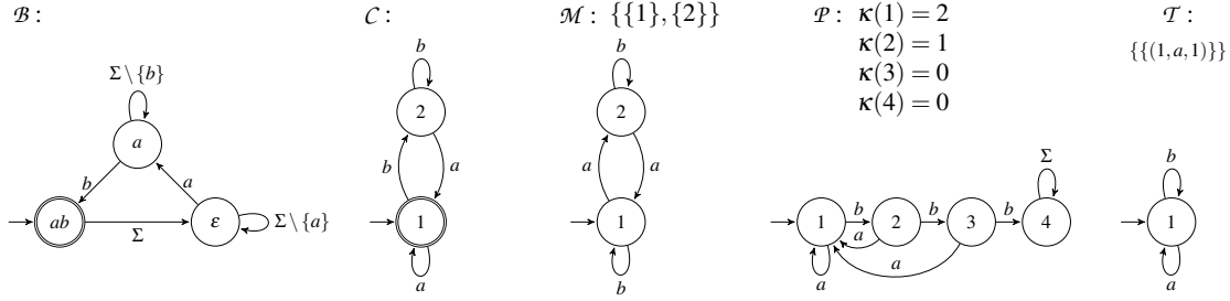
Figure 2: A DBA \mathcal{B} accepting (\Sigma^* a \Sigma^* b)^\omega where \Sigma = \{a, b, c\} , a DCA \mathcal{C} accepting (a+b)^* b^\omega , a DMA \mathcal{M} accepting (a+b)^* b^\omega , a DPA \mathcal{P} accepting (a+ba+bba)^*(a^*ba)^\omega , and a DTA \mathcal{T} accepting (a+b)^* a^\omega .
