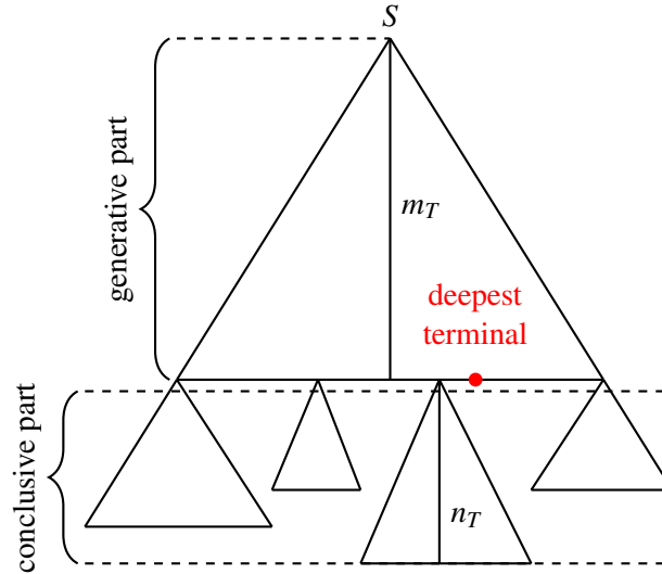
Figure 1: Separation of derivation tree, T , into the generative and conclusive part based on the deepest (lowest rightmost) terminal; all symbols located to its right are nonterminal. The conclusive part starts with the following level, and contains no terminals. No symbol belongs to both generative and conclusive parts; m_T and n_T denote the depth of the generative and conclusive part, respectively.
