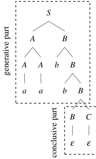
Figure 2: Derivation tree T of H for aabb where the root is S
